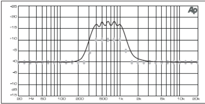
Graphic equalizer without frequency response correction.
