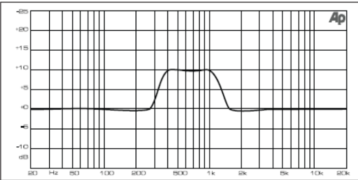
Graphic equalizer with frequency response correction.
